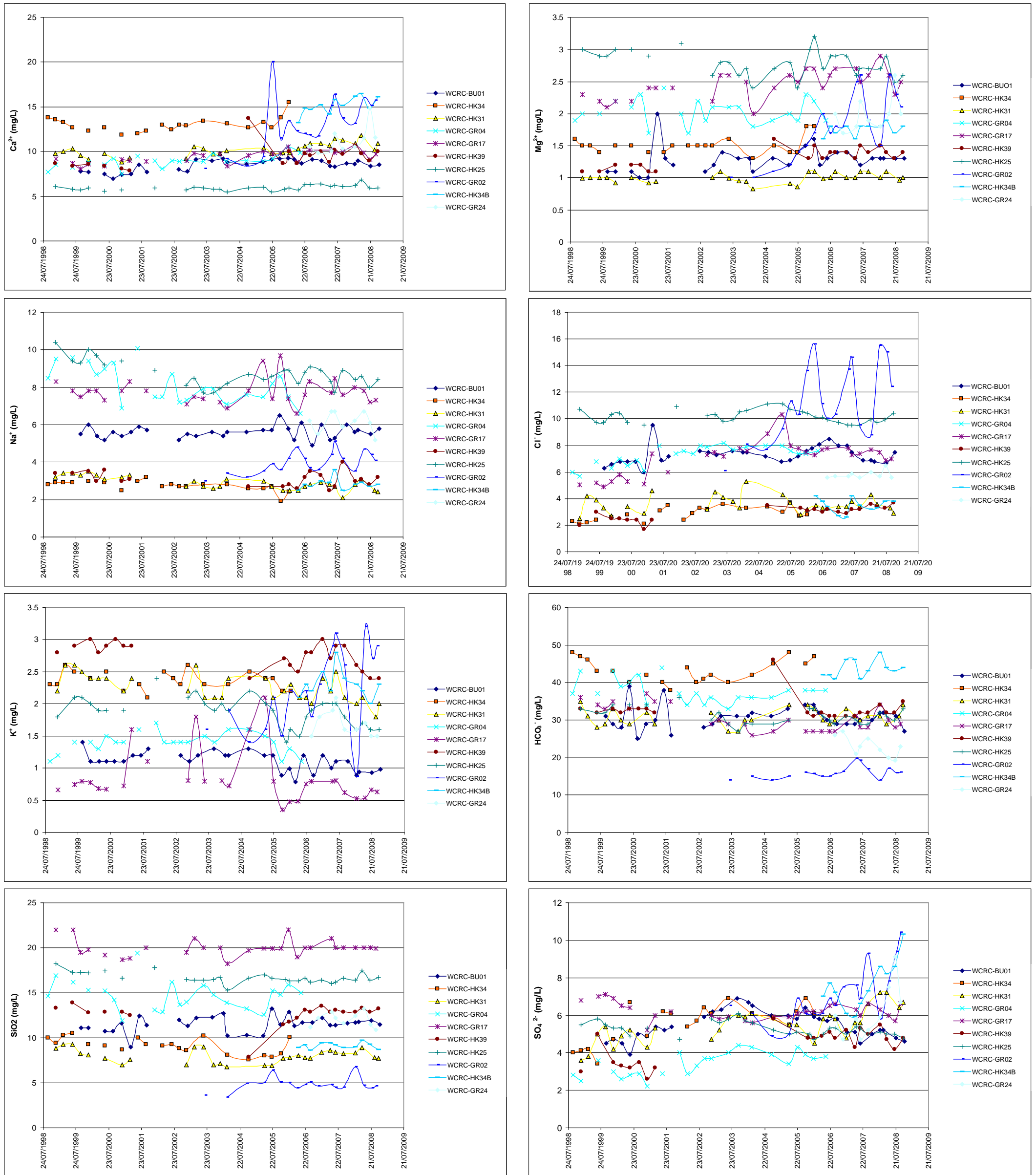
Figure 7 Time-series plots for selected water quality parameters on a per-site basis.
