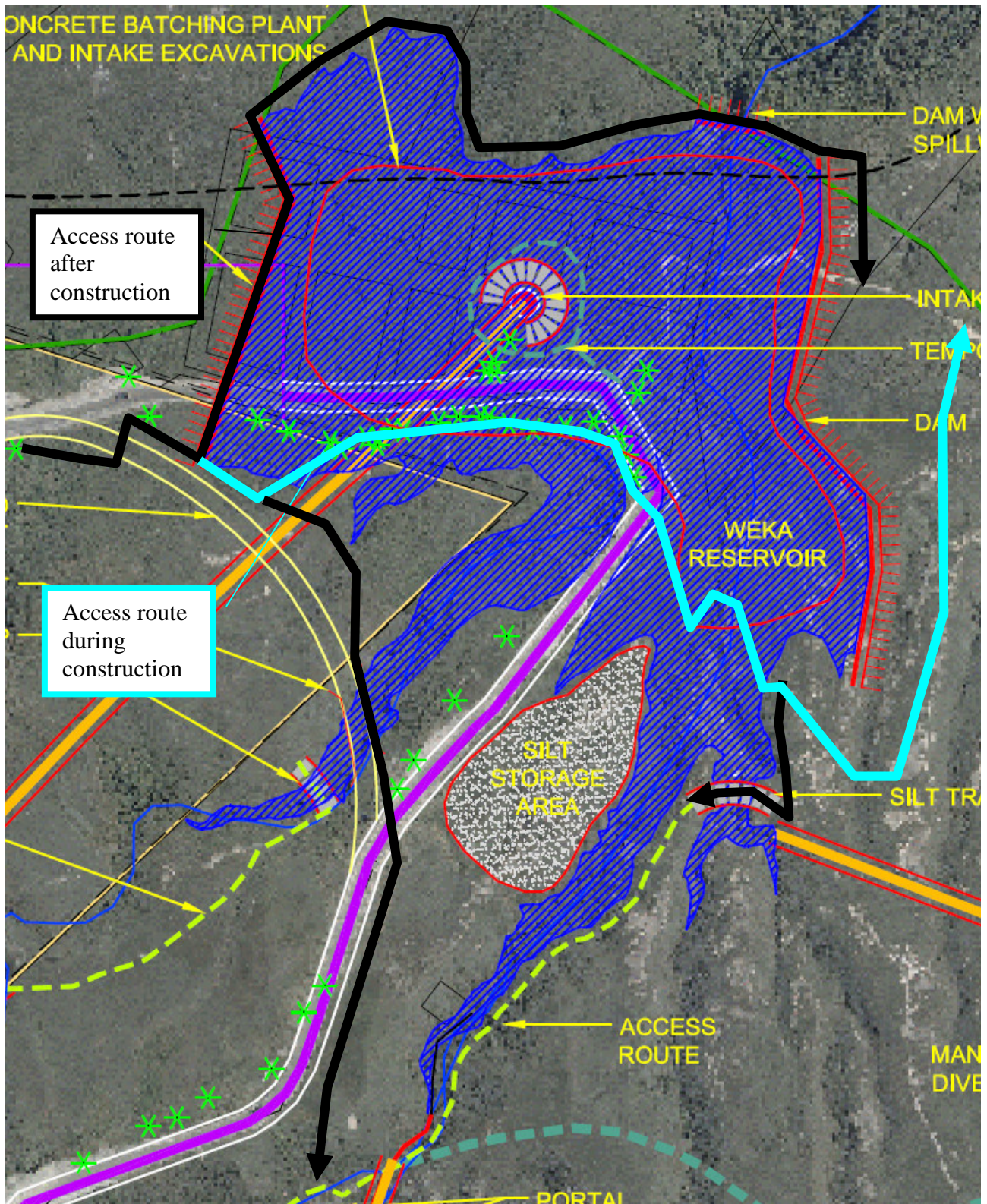
Figure showing access to the Repo basin during (blue) and following construction (black)
